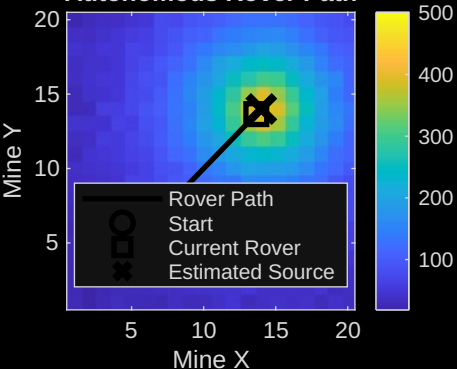
Autonomous Rover Path
